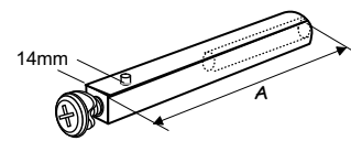
N8T-HCX Custom Half Spindle
